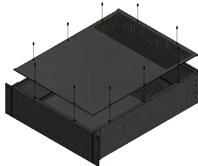
ASSEMBLY - ISOMETRIC VIEW
