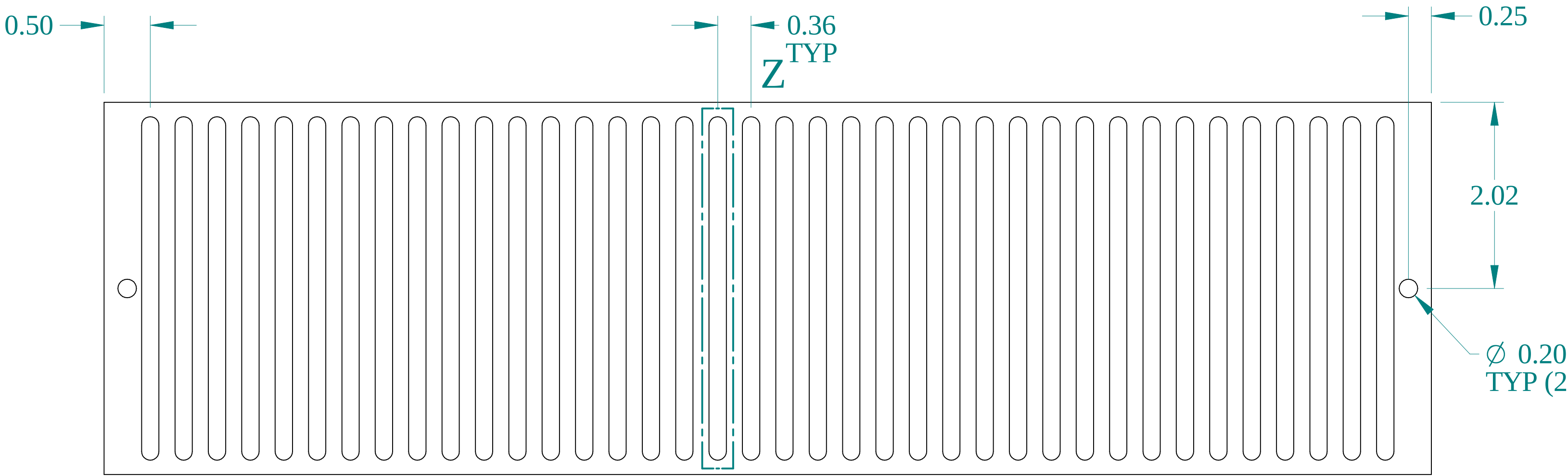
FRONT VIEW
