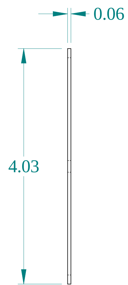
SIDE VIEW
