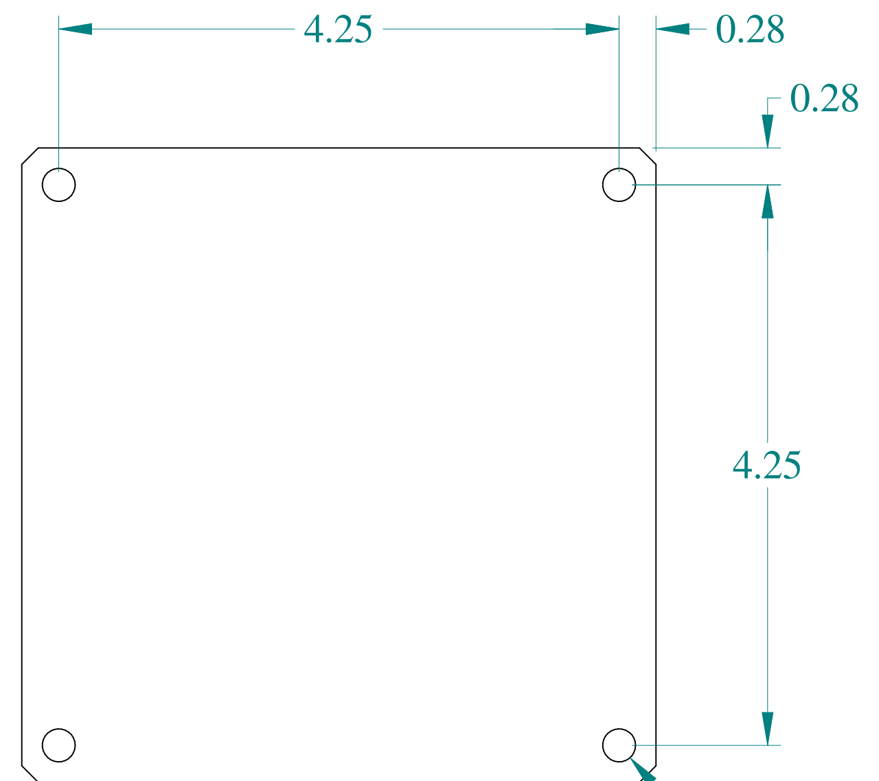
FRONT VIEW
