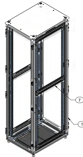
ISOMETRIC VIEW DOORS AND SIDE PANELS REMOVED
