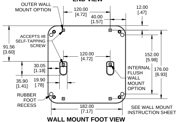
WALL MOUNT FOOT VIEW
